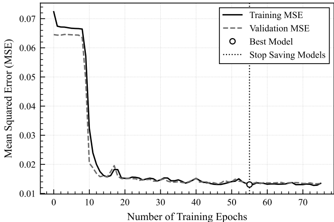
Learning Curve of TCSA-Transformer Model for SolarPlant-2 (Gyeongju)
